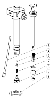
721260 Fuel Pump (for MultiFuel & OmniFuel)
