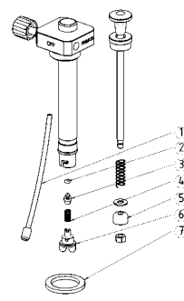
721550 Fuel Pump (for VariFuel)
